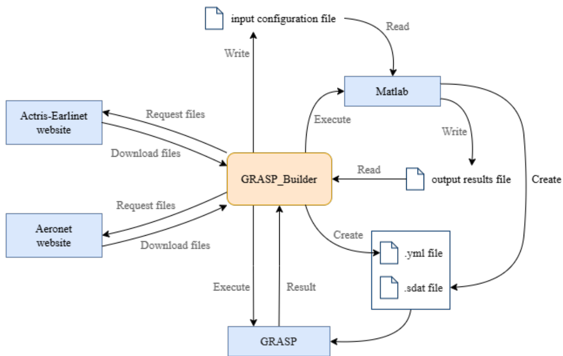
Figure 20: Application interactions diagram
