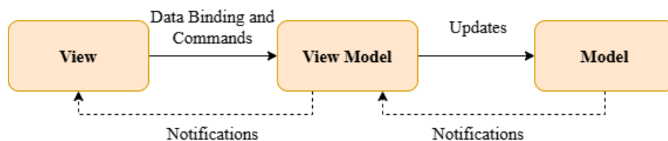
Figure 10: MVVM design pattern
